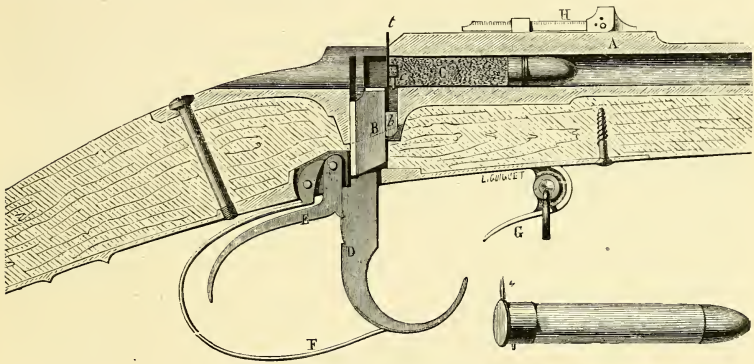
Early French Military Breech-loader.
